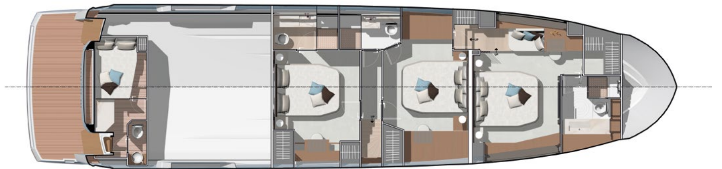
Lower deck - 3 Stateroom version
