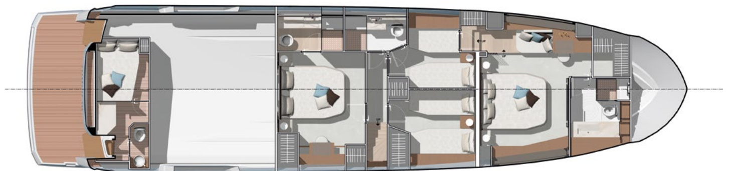
Lower deck - 4 Stateroom version
